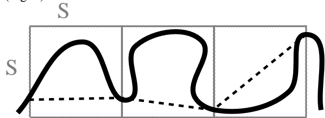
Fig. 8 Distance field sampling error. In the worst case, the actual SV boundary (heavy line) could fluctuate wildly between the grid points. The inaccuracy of the resulting approximation (dashed line) is limited by the size of the grid cell, S .
