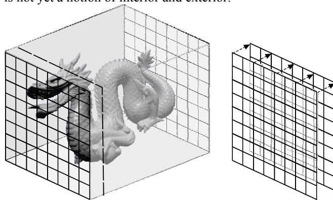
Fig. 2 The workspace is split into slices, and depth measurements performed for each slice. On the left, the dragon model is shown inside a bounding box. That box is split (right), and for each slice (such as from the front to the dashed line), distance fields are taken along the split direction.
