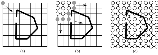
Fig. 5 The advancing front enters holes, rendering Marching Cubes useless. The front, represented by grey circles, starts at the upper left corner in (a), moving down and to the right. In (b), the front has advanced up to the hole in the volume. By the time the front is exhausted, in (c), it has completely filled the space. By labeling all the visited points Outside , it is impossible to recover the correct surface. Although the hole is exaggerated here for the purposes of example, the same phenomenon is found with the smallest of imperfections in common PLM models.
