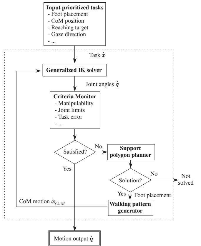
Fig. 2. Method overview
